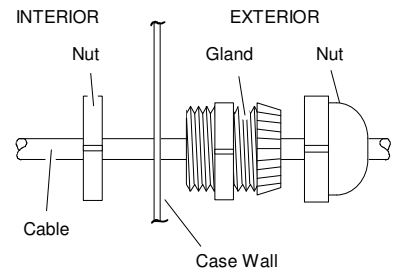
Figure 2-3. Cable Gland
